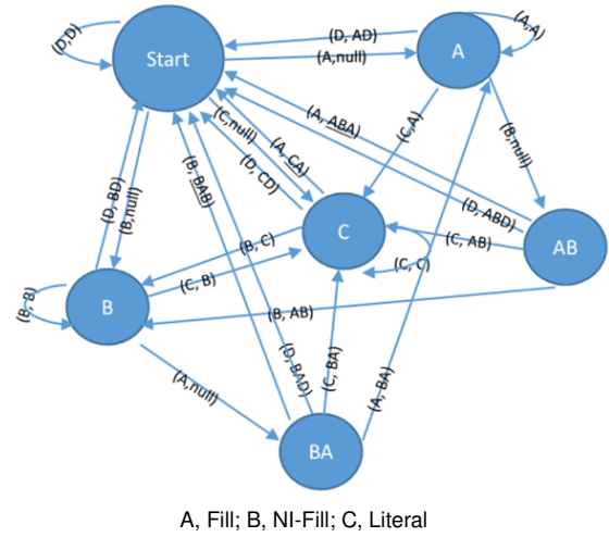
Fig. 10 Encoding automaton in ICX.
