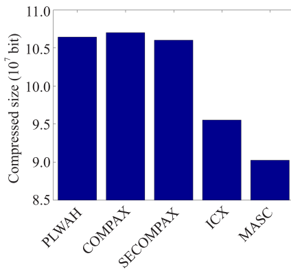
Fig. 17 Size after compression using five encoding schemes in srcPort.
