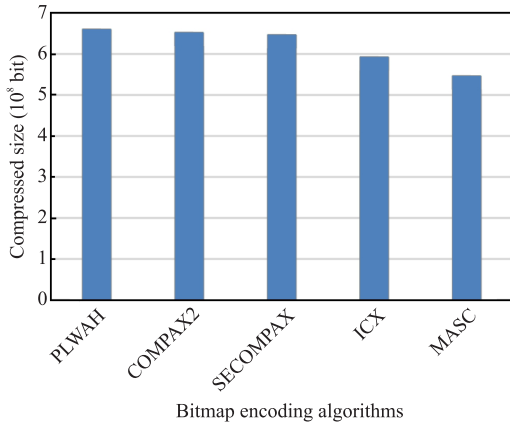
Fig. 13 Bitmap index encoding with PLWAH/COMPAX2/SECOMPAX/ICX/MASC.
