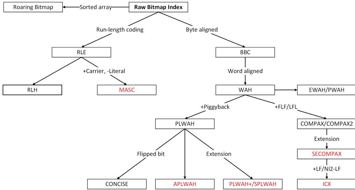
Fig. 8 New ideas in bitmap index encoding.
