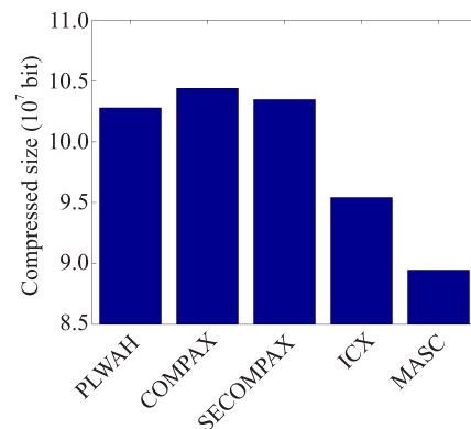
Fig. 15 Size after compression using five encoding schemes in DstPort.
