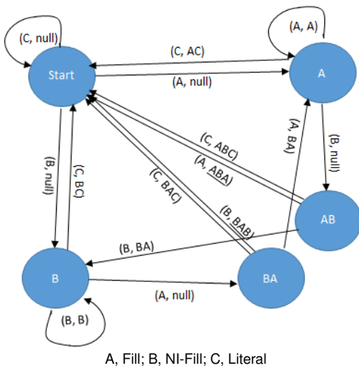
Fig. 9 Encoding algorithm of SECOMPAX. (x, y) means the next character is x , and the output is y except if y =null, output nothing, and if y is underlined, the output is a codeword as a whole.
