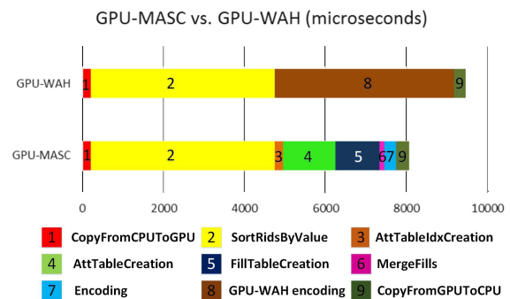
Fig. 19 Encoding time of GPU-WAH and GPU-MASC.
