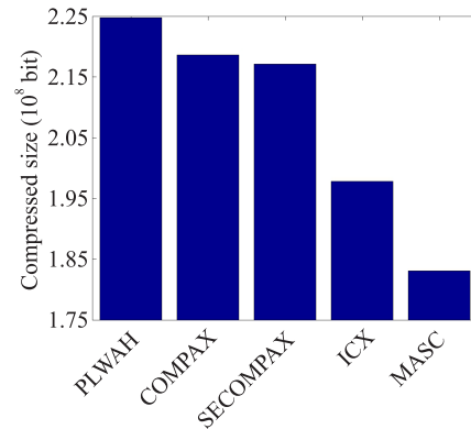
Fig. 14 Size after compression using five encoding schemes in DstIP.
