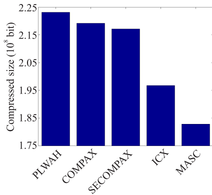
Fig. 16 Size after compression using five encoding schemes in SrcIP.
