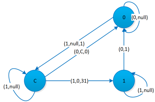
Fig. 11 Encoding automaton in MASC. States 0: 0-Fill; 1: 1-Fill; and C: 1-carried-0-Fill (0-Fill word carried 1’s). The meaning of transfer edge (x, y, z) is as follows: x , input bit (0 or 1); y , output bit; z , the counter. If label (x, y) does not occur, the counter will increase by 1, by default.
