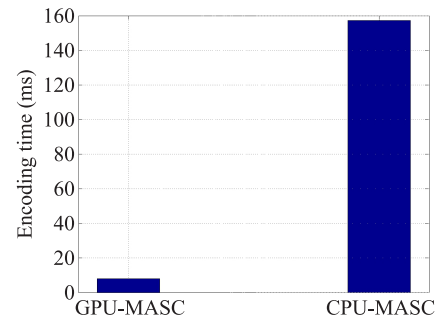
Fig. 18 Encoding-speed comparison between GPU-MASC and CPU-MASC.
