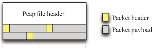
Fig. 1 Pcap file format.
