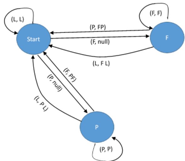
Fig. 12 Encoding automaton in PLWAH+. “Start” is the start state of a compression procedure, symbol “F” stands for codeword Fill word, symbol “P” stands for codeword NI word, and symbol “L” stands for codeword Literal word.
