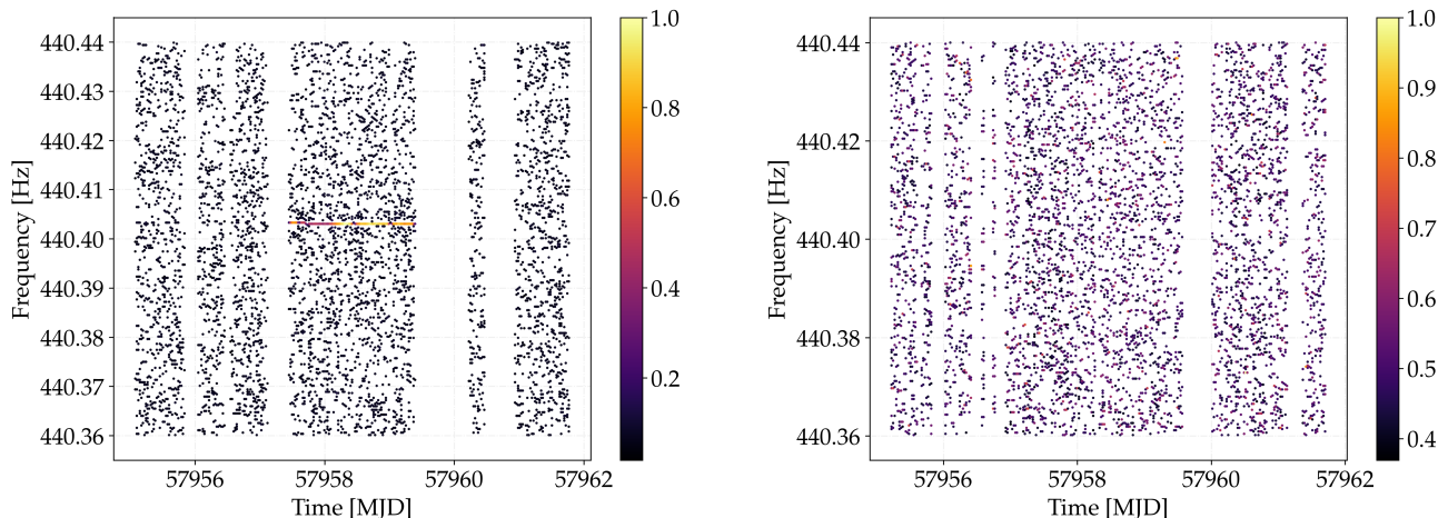
FIG. 5. FrequencyHough peakmaps, without Doppler correction, around the outlier at \sim 440.4 Hz, for Hanford (left) and Livingston (right) data. The presence of a transient line is clearly visible in Hanford. The x-axis indicates time in Modified Julian Date (MJD).
